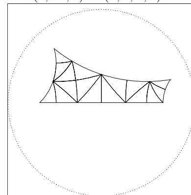
Case C18: K = 16 , (4, 2, 5) \subset (2, 4, 5, 4)
