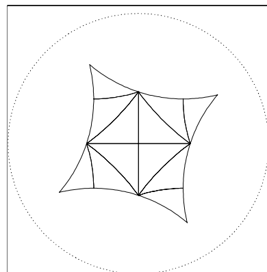
Case C12: K = 12 , (5, 2, 5) \subset (5, 5, 5, 5)
