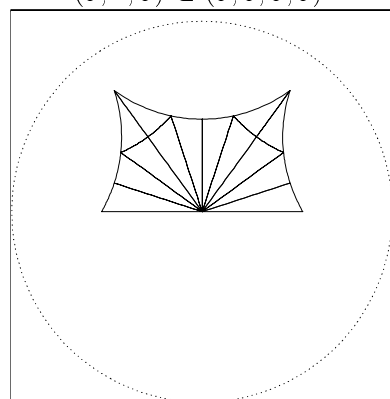
Case C15: K = 14 , (3, 10, 2) \subset (3, 3, 5, 5)
